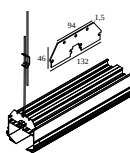
420 52 98 01 SPM52 - SUSPENSION BRACKET
